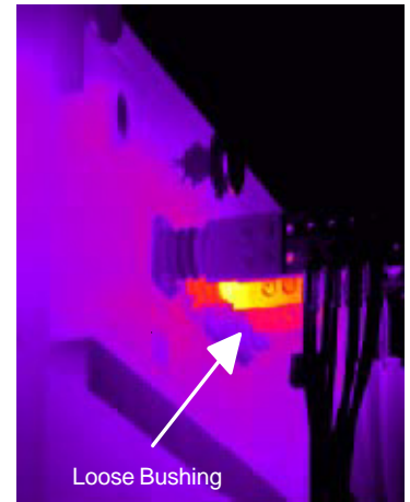
Electrical Equipment IR P/PM
