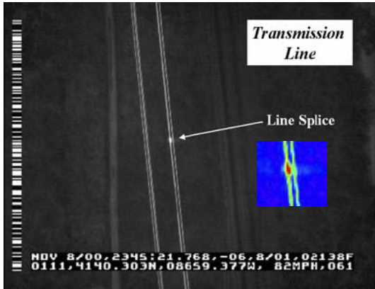
Aerial Electrical Infrared on Transmission Line
