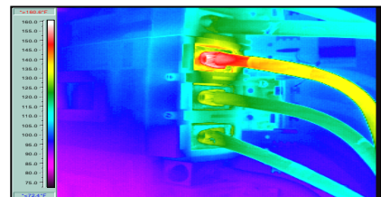
Infrared Photo showing electrical fault due to loose connection.
